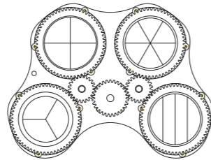
Prism 1: 4 different prisms, 4-Facet linear prism/3-Facet circular prism/4-Facet circular prism/6-facet circular prism with variable speed and direction
