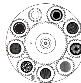
Rotating gobo
